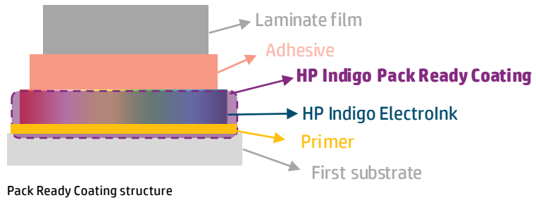
Pack Ready Coating structure
