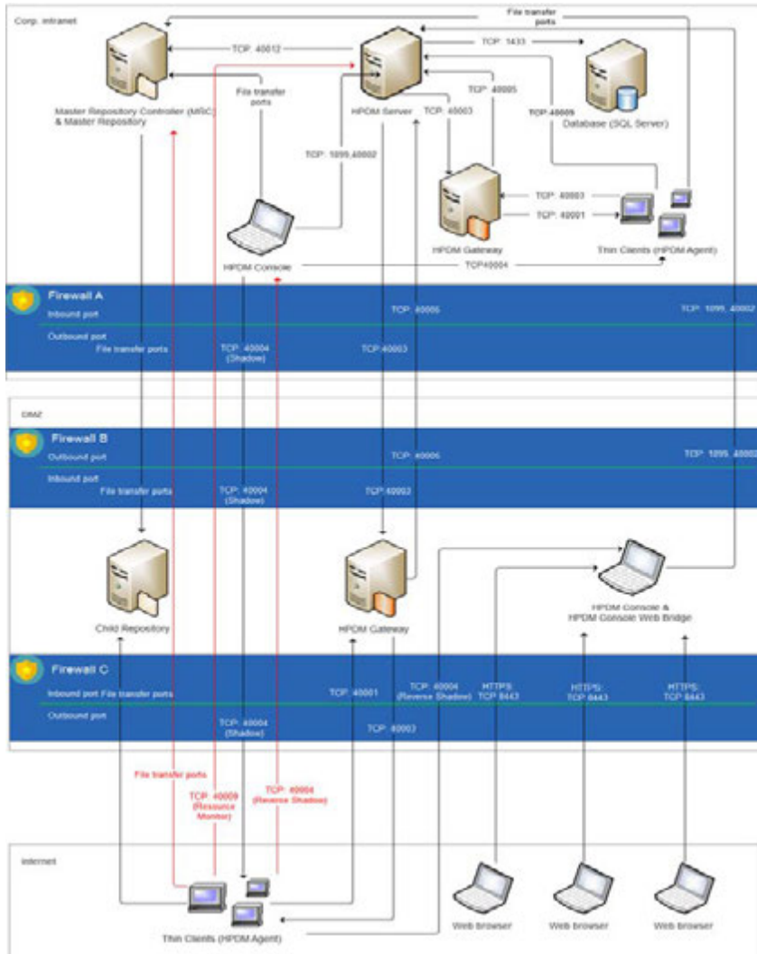
Figure 5. Typical HPDM topology in a DMZ environment
